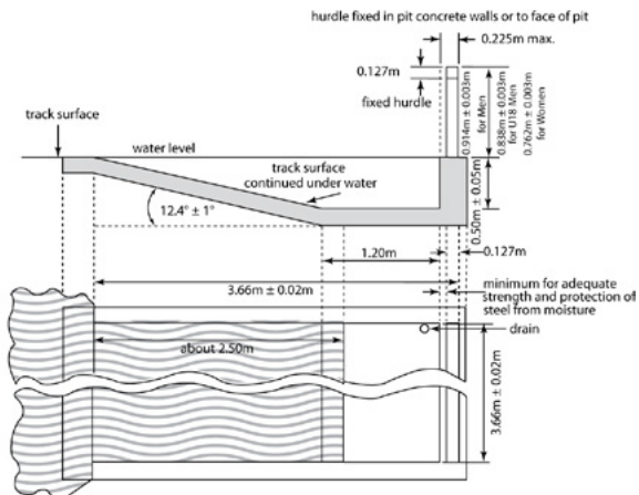
Figure (b) TR23 – Water jump
