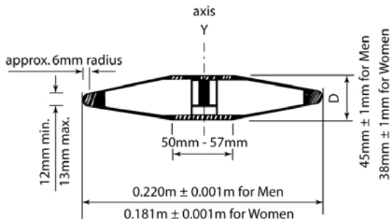
Figure TR34 – Discus
