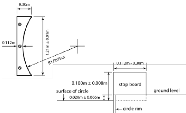
Figure TR33 – Shot Put stop board (top and side view)
