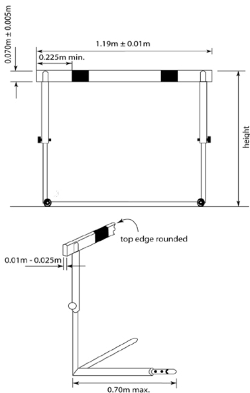
Figure TR22 – Example of a hurdle
